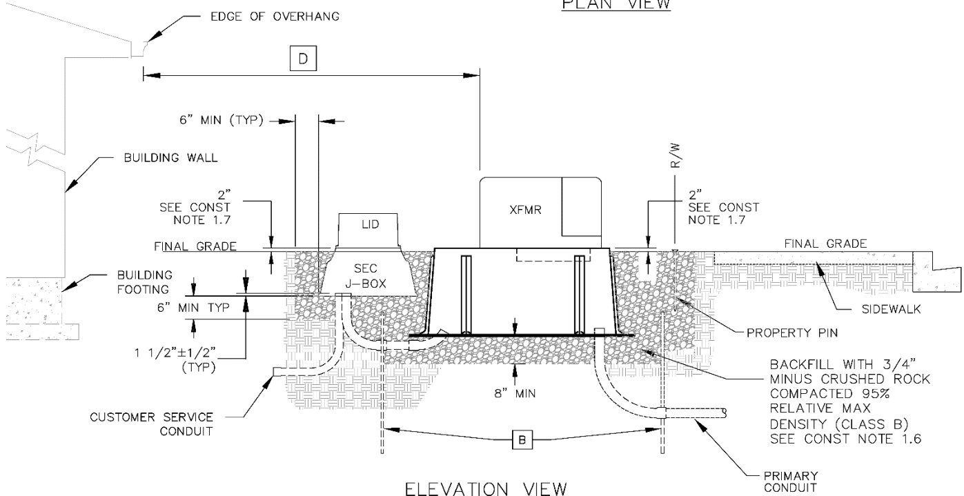
ELEVATION VIEW
